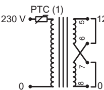
Secondary 12V parallel coupling
