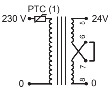
Secondary 24V serial coupling
